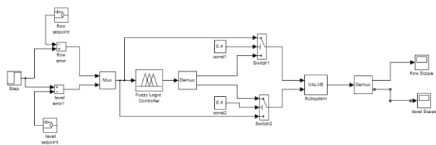
Fig.8. The structure diagram of the fuzzy control system of storage tank
