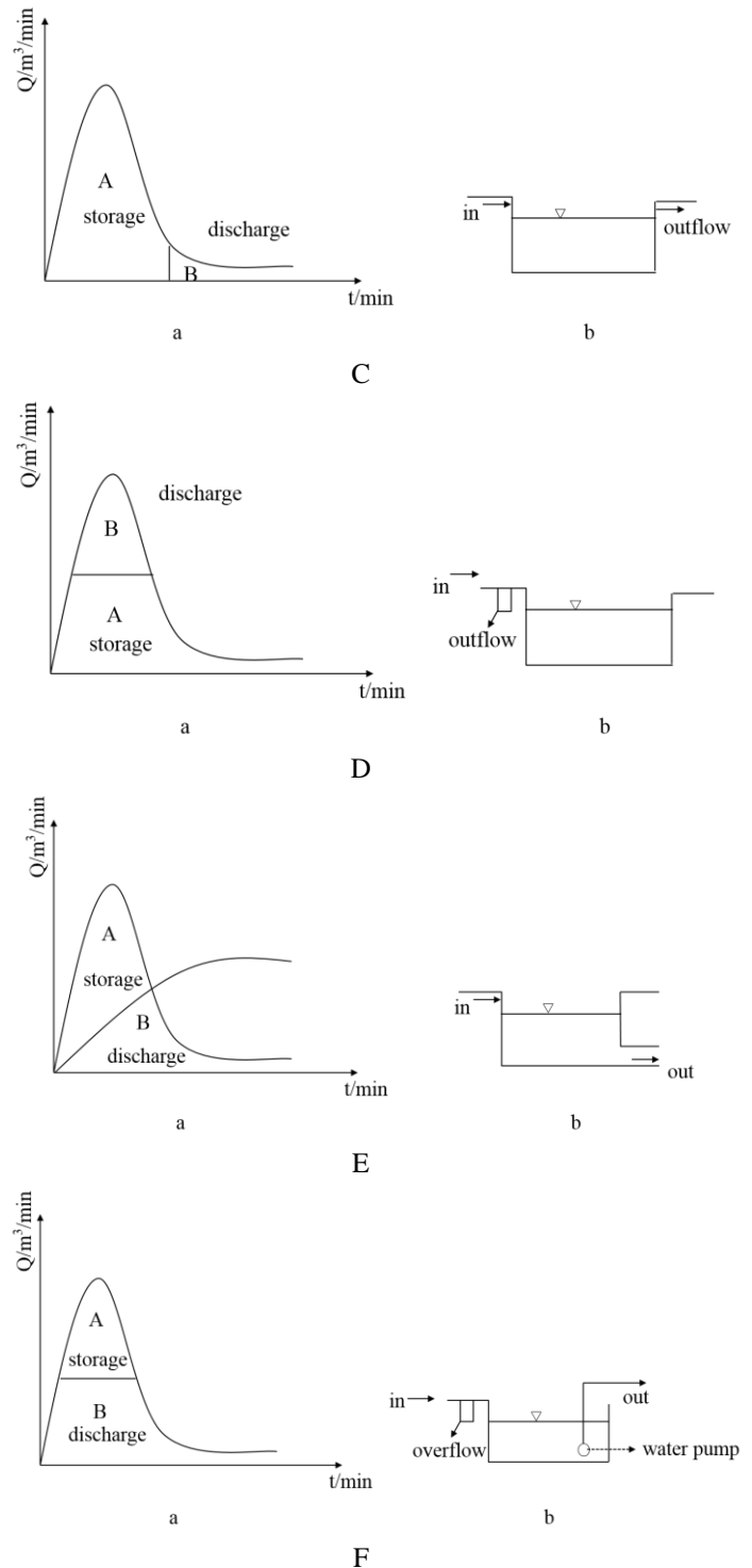
Fig. 1. The simplified model of storage tank based on reducing the stormwater runoff (A and B are the storage and discharge of the stormwater runoff respectively; a and b are the hydrologic progress curve and the simplified model of storage tank respectively; C and D are the storage tank based on the stormwater harvesting and E and F are the storage tank based on regulating flood peak.)
