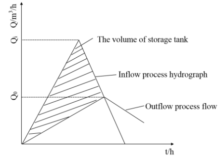
Fig.5. Schematic diagram of the triangular hydrograph method ( Q_i is the inflow peak flow and Q_0 is the outflow peak flow.)
