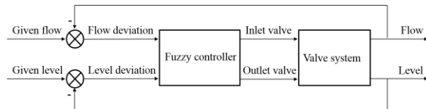
Fig.7. The structure diagram of the fuzzy control system
