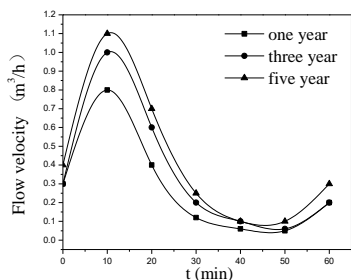
Fig.3. The flow velocity under different return periods
