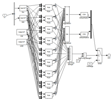
Fig.9. The structure diagram of the fuzzy control rule of the storage tank
