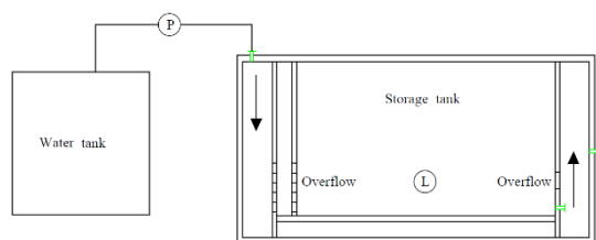
Fig. 2. The simulated experimental device of storage tank (P is the water pump; the arrow direction is the flow direction; L is the online water level meter)
