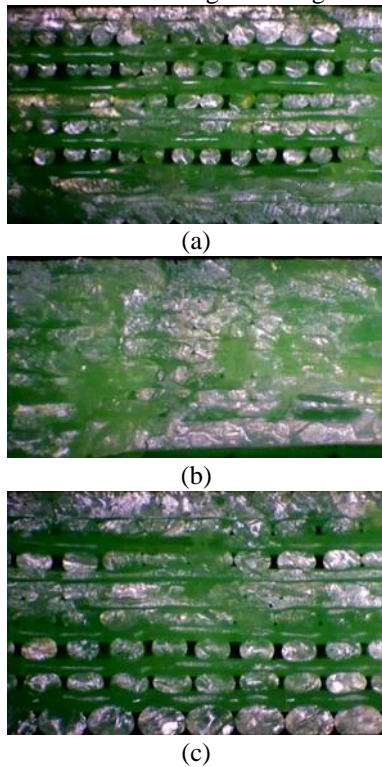
Fig. 9 Fractured surface of specimen at (a) 400 μm, (b) 500 μm and (c) 600 μm raster width
