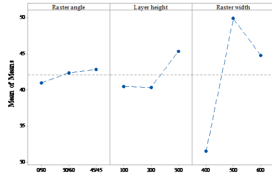
Fig. 3 Main effect plot of S/N ratio for tensile strength
